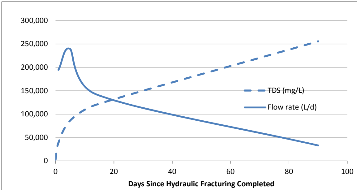
Figure 7. Change in the Total Dissolved Solids Concentration of Produced Fluids over Time (example of a Marcellus Shale well)
