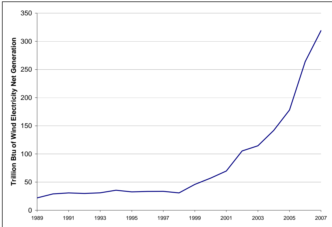
Figure 20. Wind Electricity Net Generation, 1989-2007
