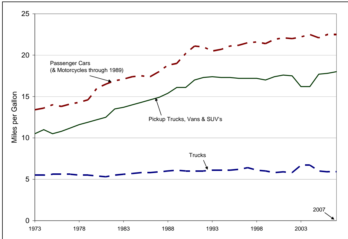
Figure 21. Motor Vehicle Efficiency Rates, 1973-2007
