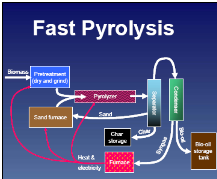
Figure 2. Biochar Production via Pyrolysis
