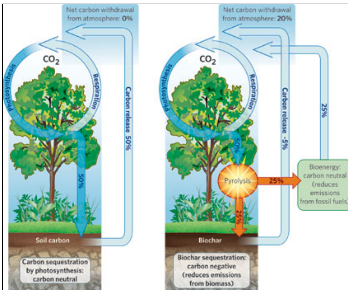
Figure 3. Carbon Cycle for Soil Carbon and Biochar
